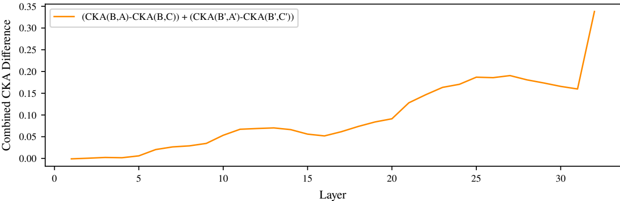
Combined CKA Difference for Llama-2-7B
