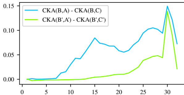
Independent Components (CKA)
