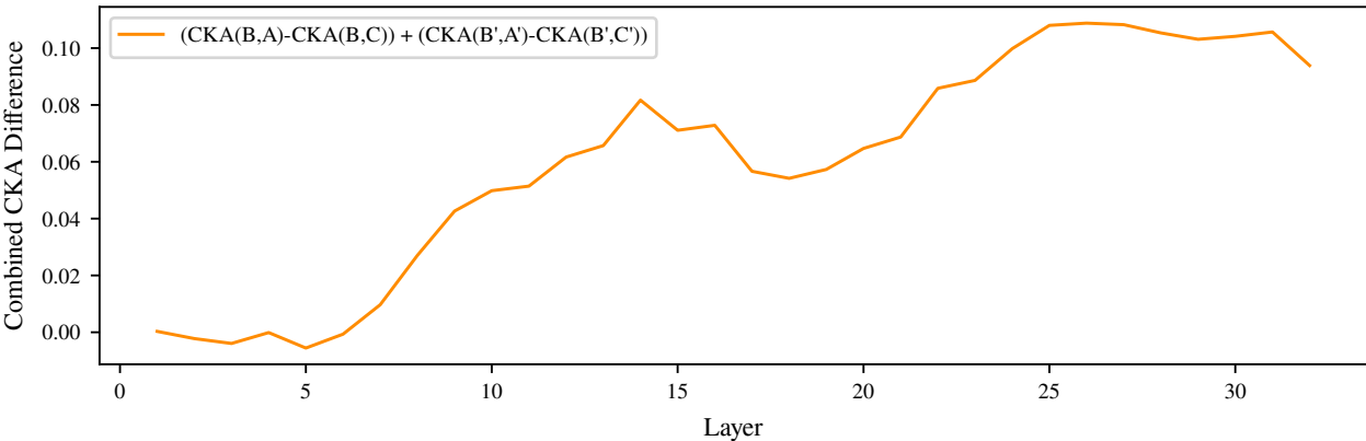
Combined CKA Difference for Mistral-7B-Instruct-v0.1
