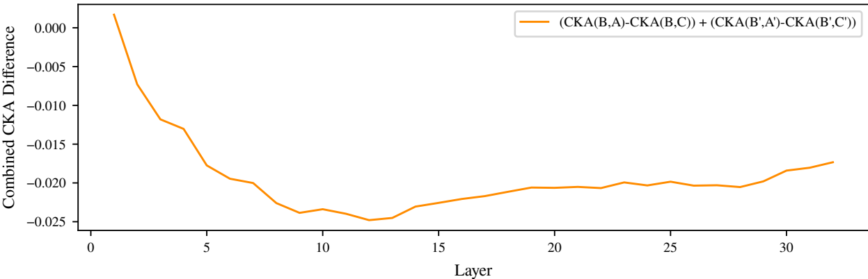
Combined CKA Difference for Phi-3.5-mini-instruct
