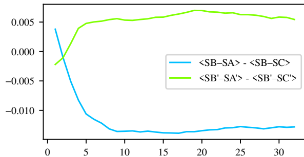
Independent Components
