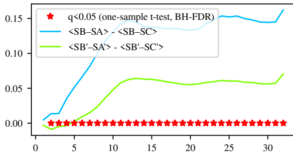
Independent Components
