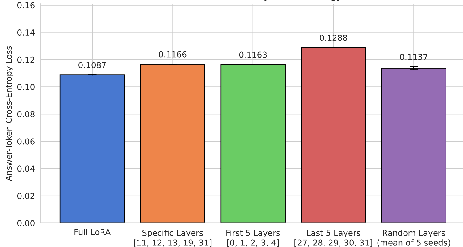
Answer-Token Loss by LoRA Strategy
