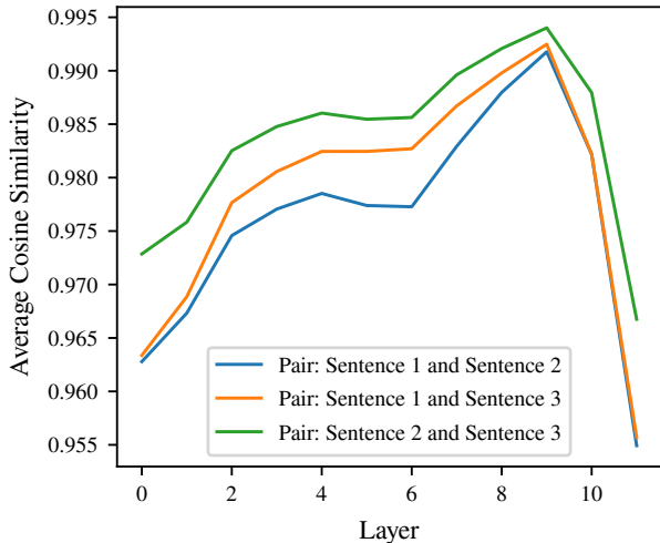
Average Cosine Similarity using the mean token embeddings for BioBERT
