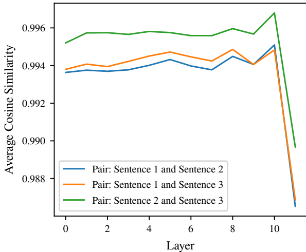
Average Cosine Similarity using the mean token embeddings for FacebookAI_roberta-base
