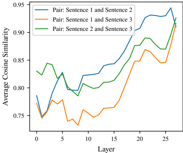
Average Cosine Similarity using the target token embeddings for Falcon
