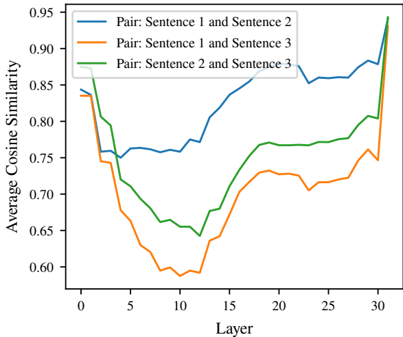
Average Cosine Similarity using the target token embeddings for Mistral
