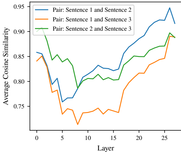
Average Cosine Similarity using the target token embeddings for Qwen_Qwen2.5-7B
