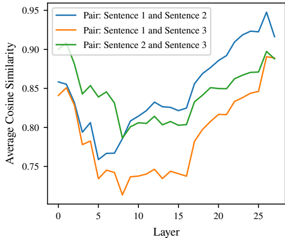
Average Cosine Similarity using the target token embeddings for Qwen
