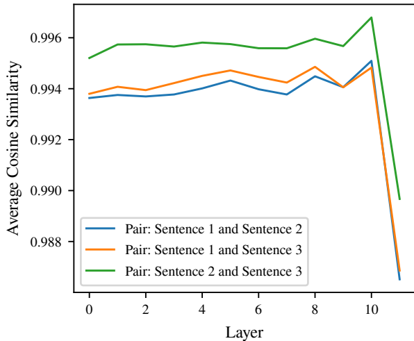
Average Cosine Similarity using the mean token embeddings for RoBERTa
