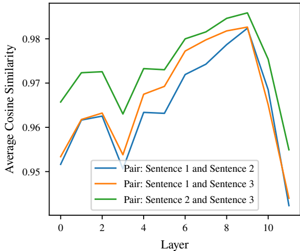
Average Cosine Similarity using the mean token embeddings for google_multibert- seed_3
