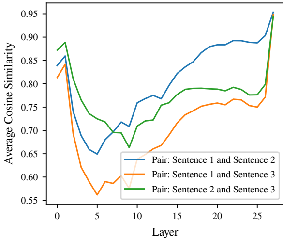
Average Cosine Similarity using the target token embeddings for meta-llama_Llama-3.2-3B
