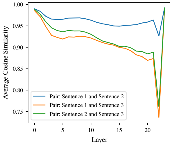
Average Cosine Similarity using the target token embeddings for microsoft_biogpt
