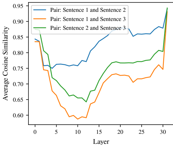
Average Cosine Similarity using the target token embeddings for mistralai_Mistral-7B-v0.1
