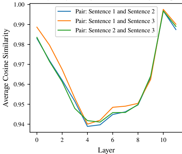
Average Cosine Similarity using the target token embeddings for openai-community_gpt2
