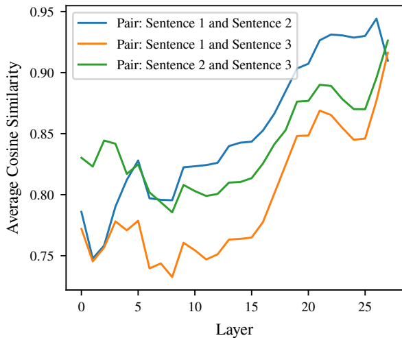
Average Cosine Similarity using the target token embeddings for tiuae_Falcon3-7B-Base
