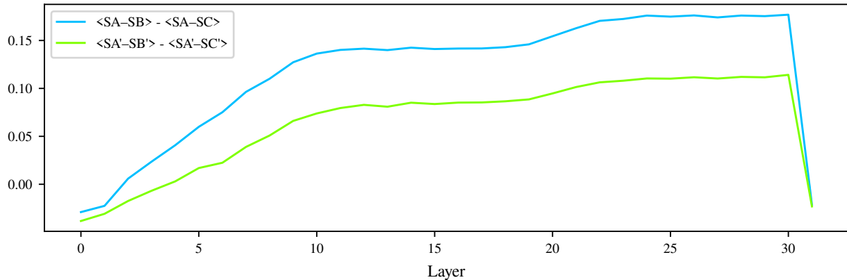
Average Difference in Cosine Similarity for Bio-Medical-Llama
