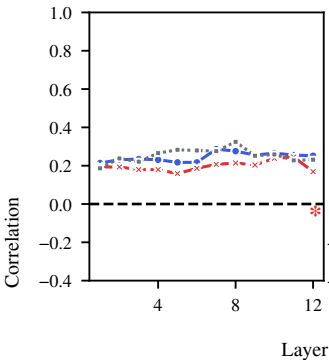
MultiBERTs
