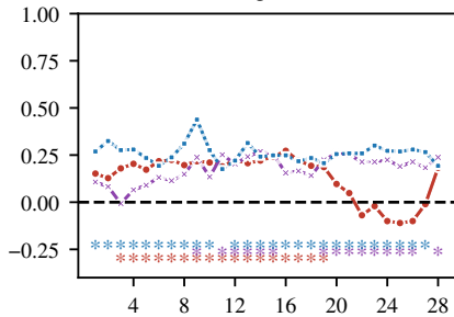
Correlation
