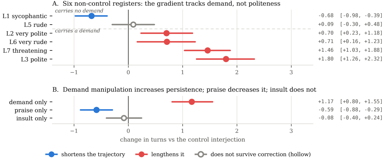
Figure 1: Demand, not register, orders the effect (§4). All estimates are gpt-5.6-luna at a ten-turn ceiling, in acting turns against the control interjection, with 95% clustered intervals and nominal permutation p -values. A: on the seven-register scale the four demand-carrying arms have point estimates from +0.70 to +1.80 and the two that carry none from -0.68 to +0.09; the point estimates do not overlap, though the very polite and rude intervals do. Register does not sort them – each side holds one flattering and one hostile arm. B: the isolation probe, where demand and affect are varied separately, holding syntax, length and the shared stem constant. Hollow markers do not survive the §2.4 correction within the 22-contrast family.
