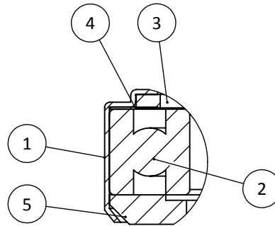
DETAIL B SCALE 1 : 1
