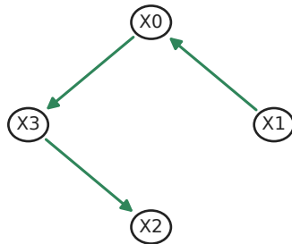
PC+greedy
