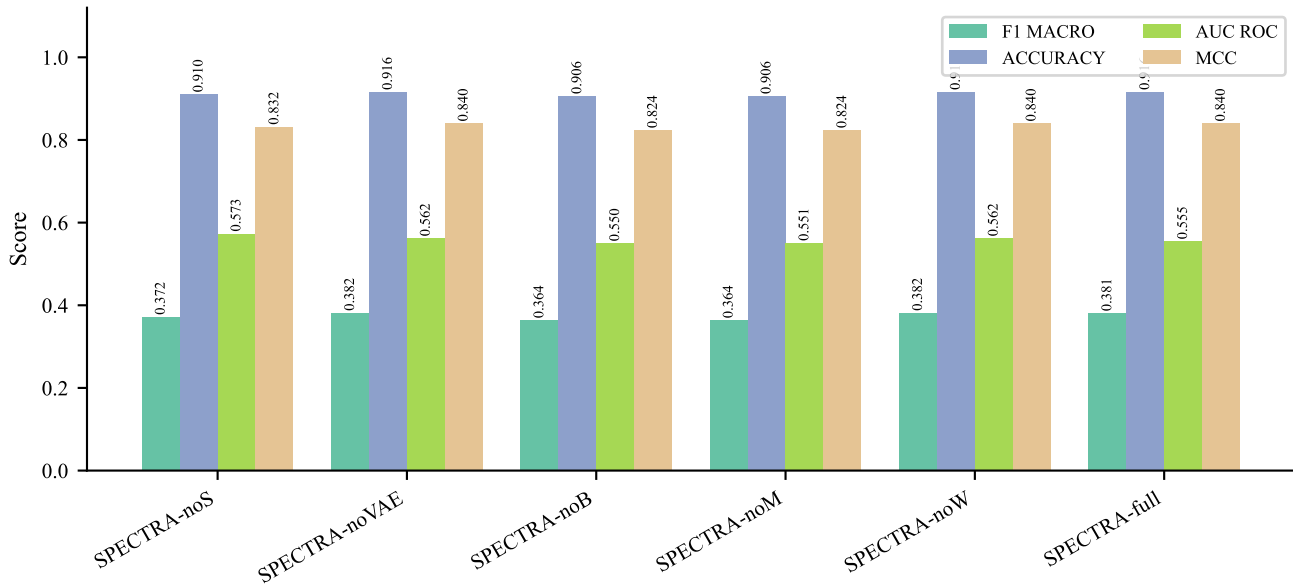
SPECTRA Ablation Study
