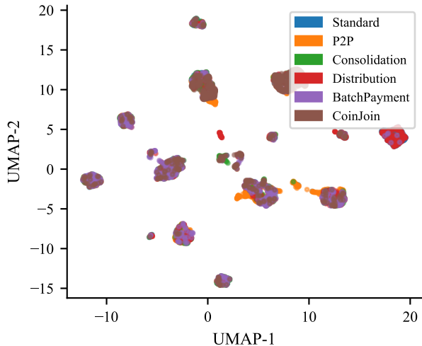
VAE Latent — Transaction Type
