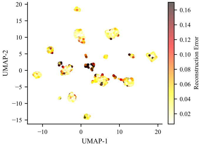
VAE Latent — Anomaly Score
