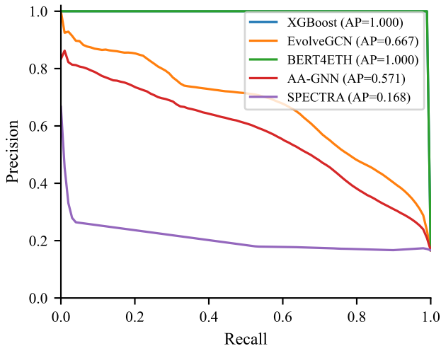
Precision-Recall Curves (Macro-Average)
