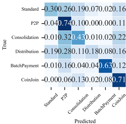
AA-GNN
