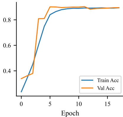
GNN Accuracy
