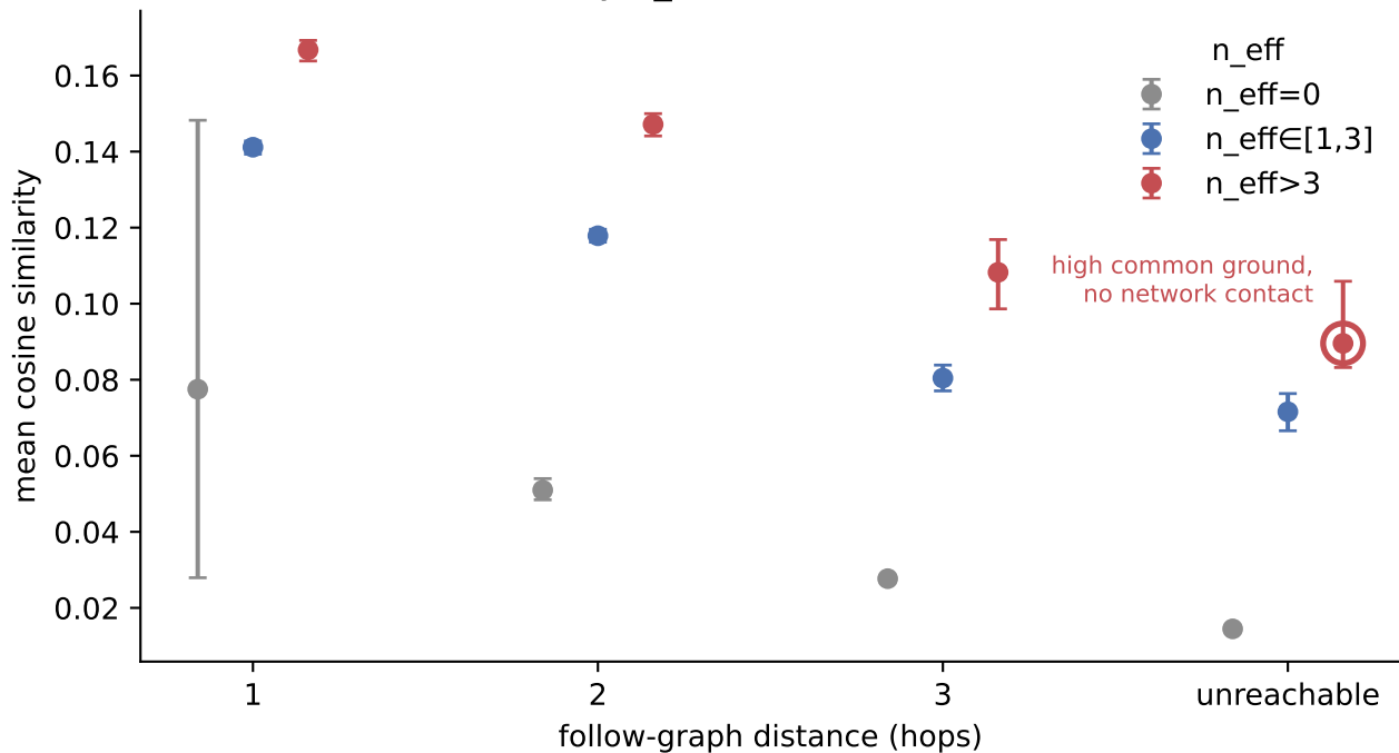
(C) mean cosine by n_eff stratum and network distance
