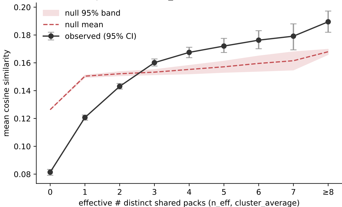
Similarity-normalized ( n_{\text{eff}} ) vs cosine (observed vs null)
