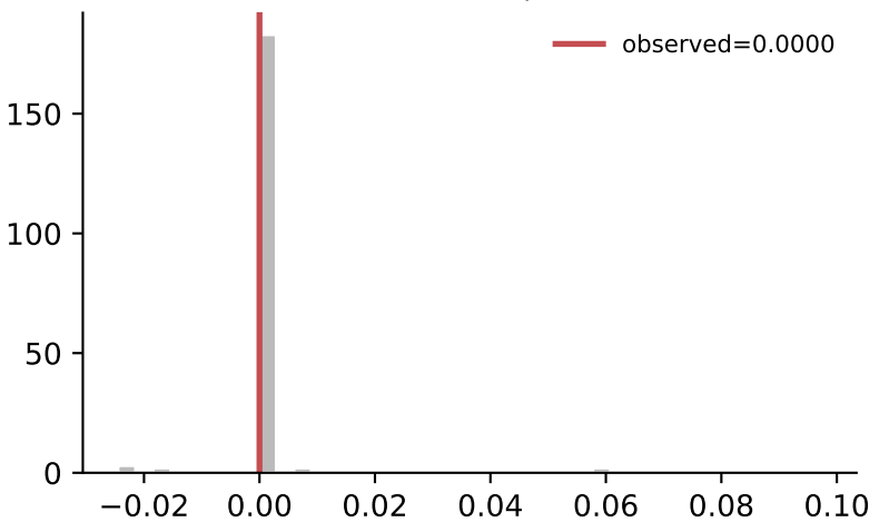
interaction[hops=4]
