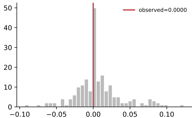
interaction[hops=3]
