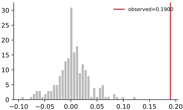
interaction[hops=2]
