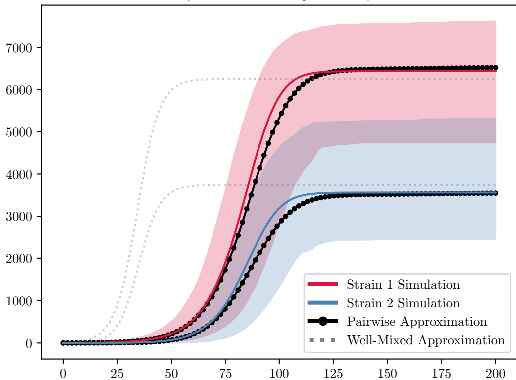
Dynamics on k-Regular Graph
