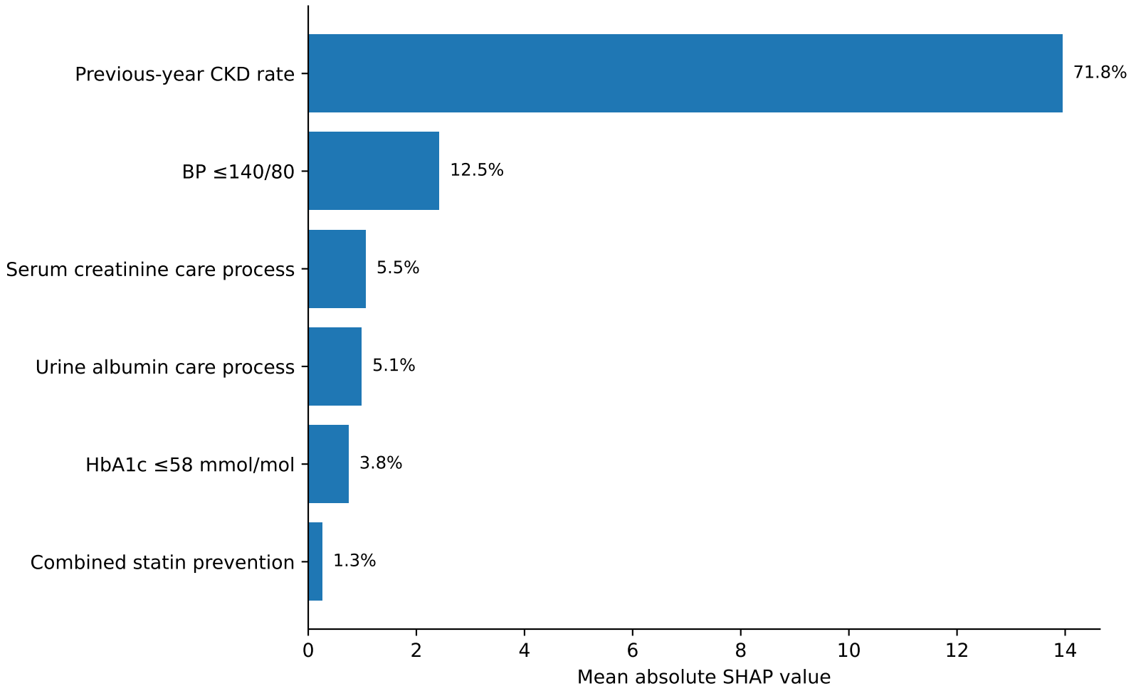
Global SHAP Importance for the Locked Ridge Model
