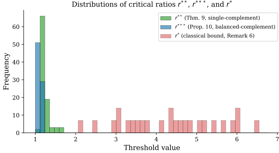
Figure S2: Histograms of r^{**} , r^{***} , and r^* over all NN instances. r^{**} and r^{***} concentrate near the empirical r (making them informative Core-emptiness thresholds via Theorem 9 and Proposition 10); r^* lies far to the right and rarely binds.
