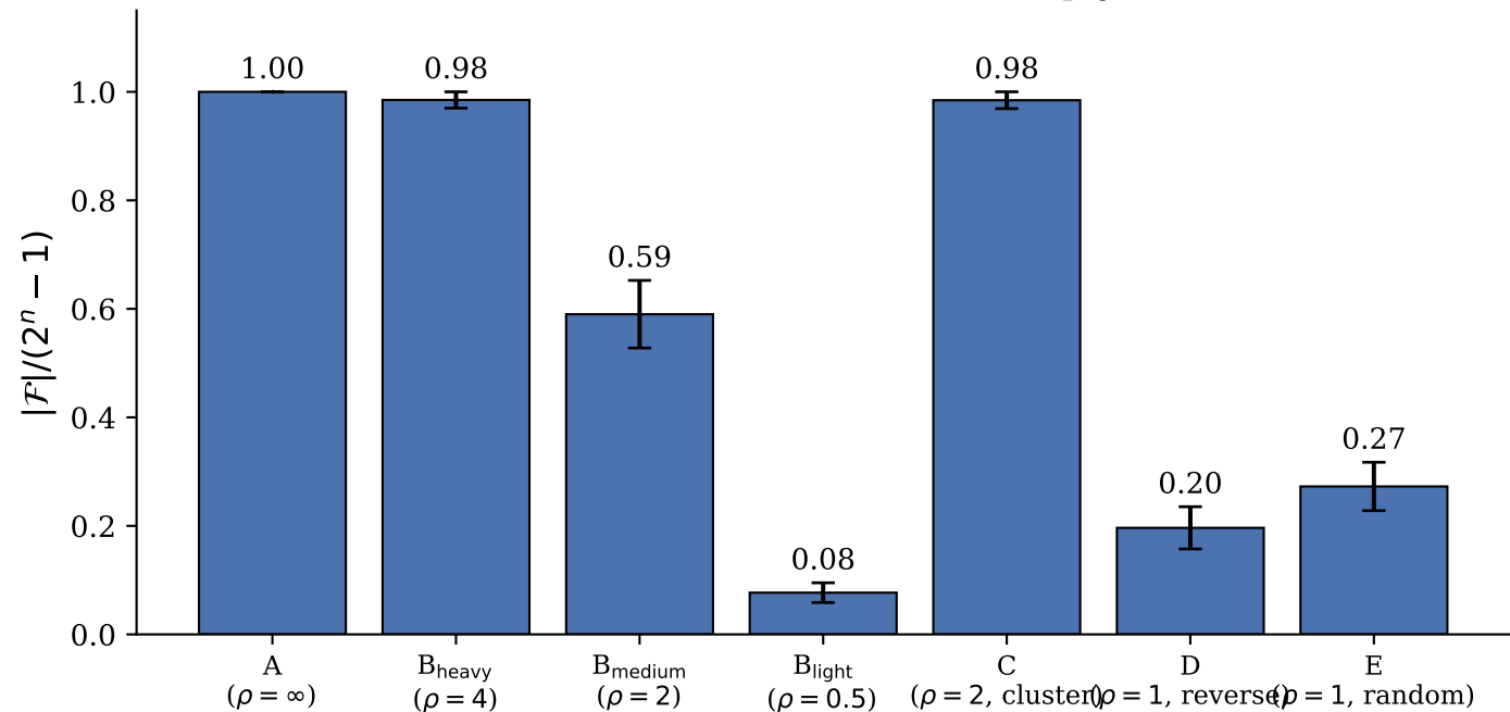
Feasible coalitions relative to all non-empty coalitions
