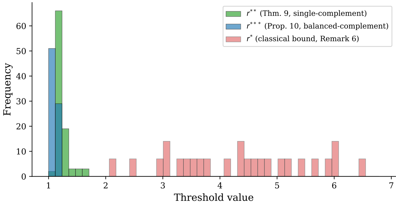
Distributions of critical ratios r^{**} , r^{***} , and r^*
