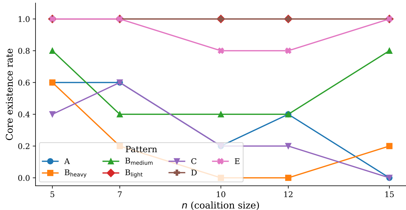
Core existence rate versus coalition size n
