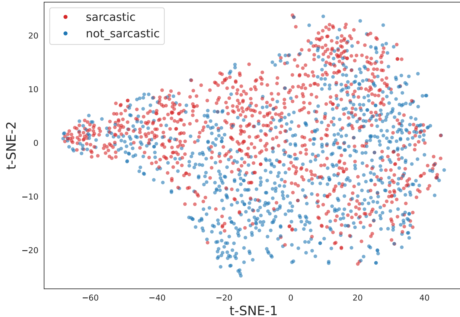
t-SNE 2D
