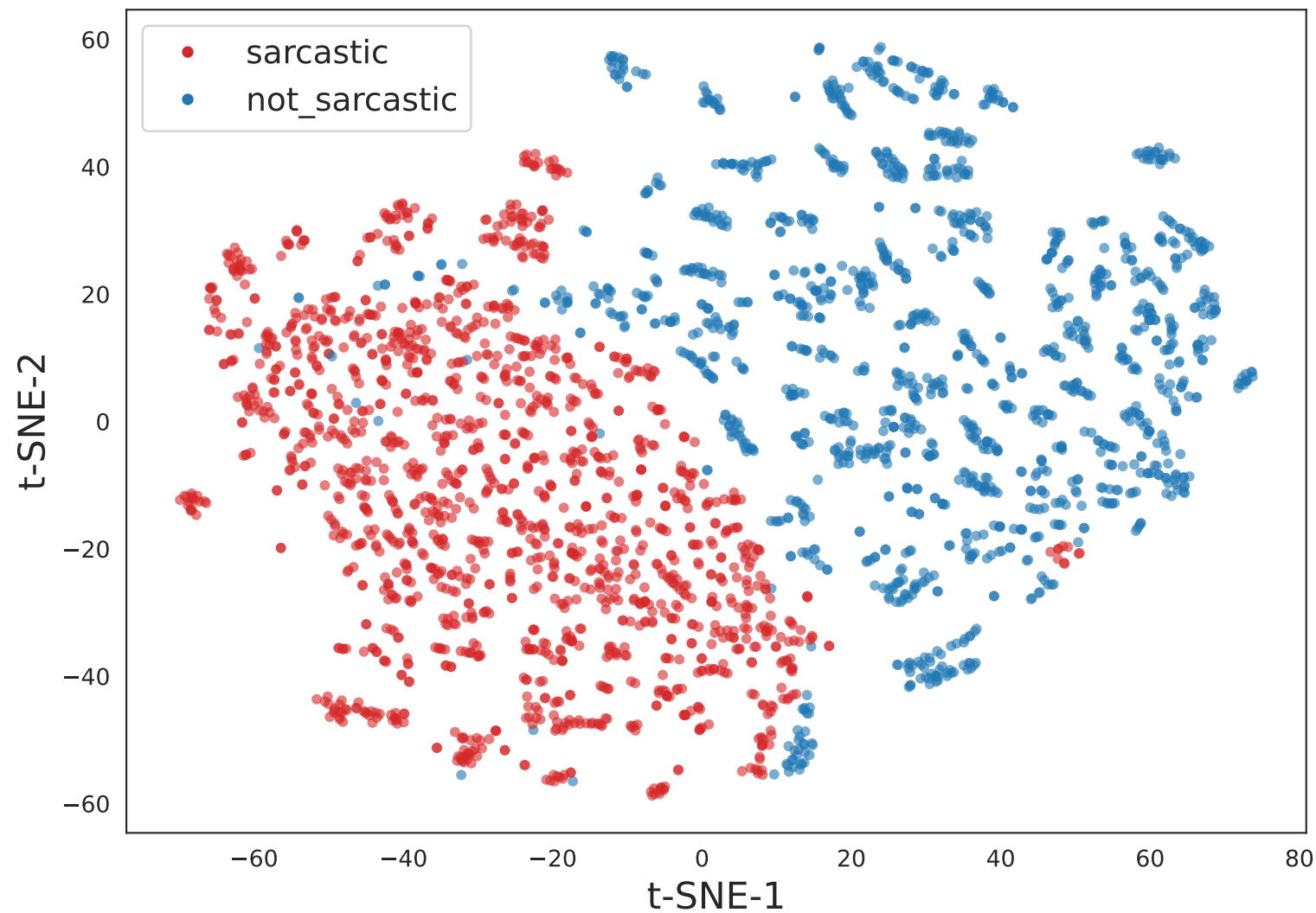
t-SNE 2D
