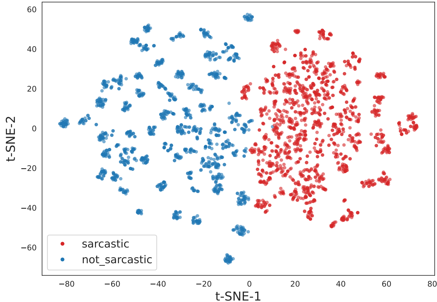
t-SNE 2D
