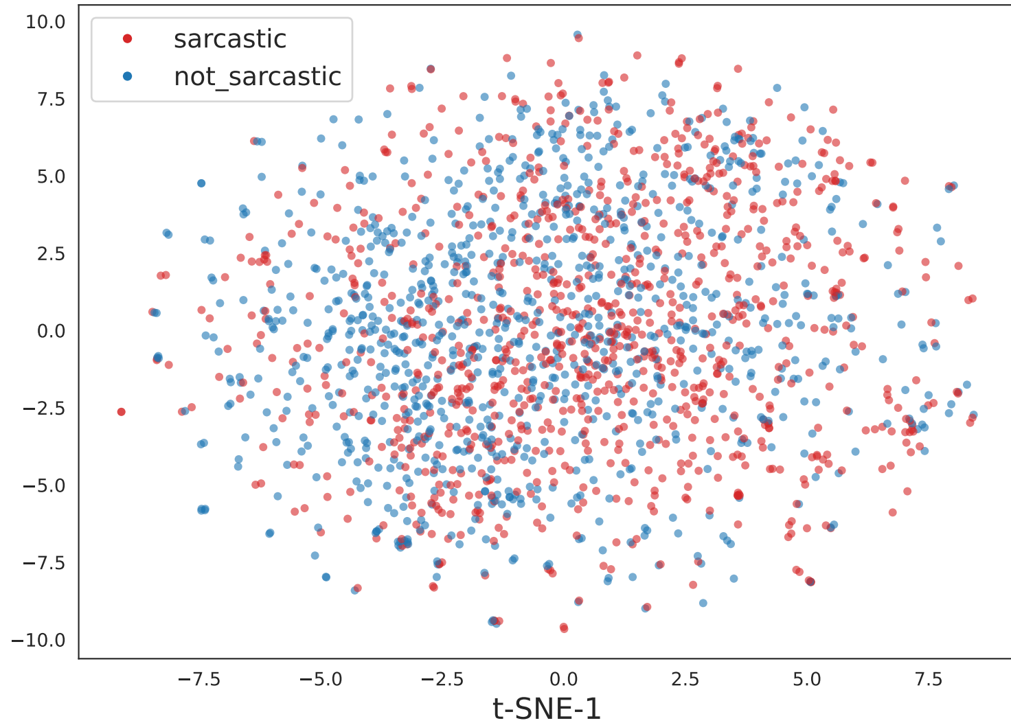
t-SNE 2D
