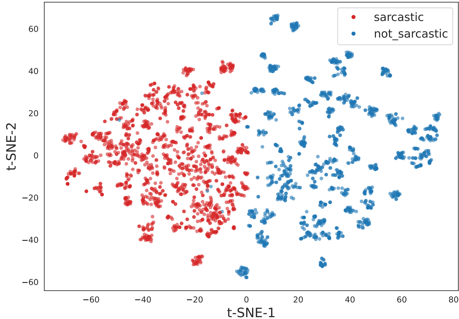
t-SNE 2D
