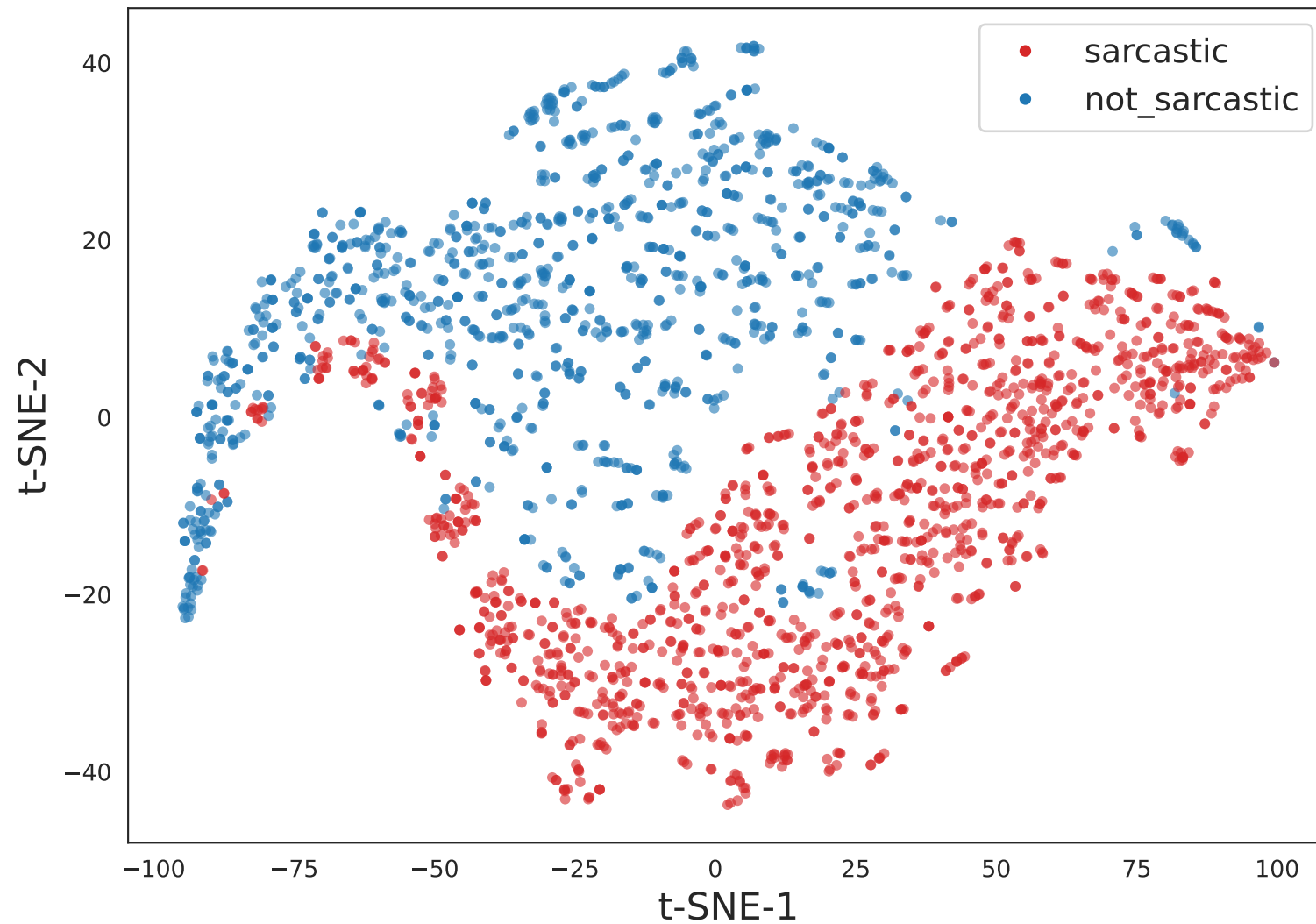
t-SNE 2D
