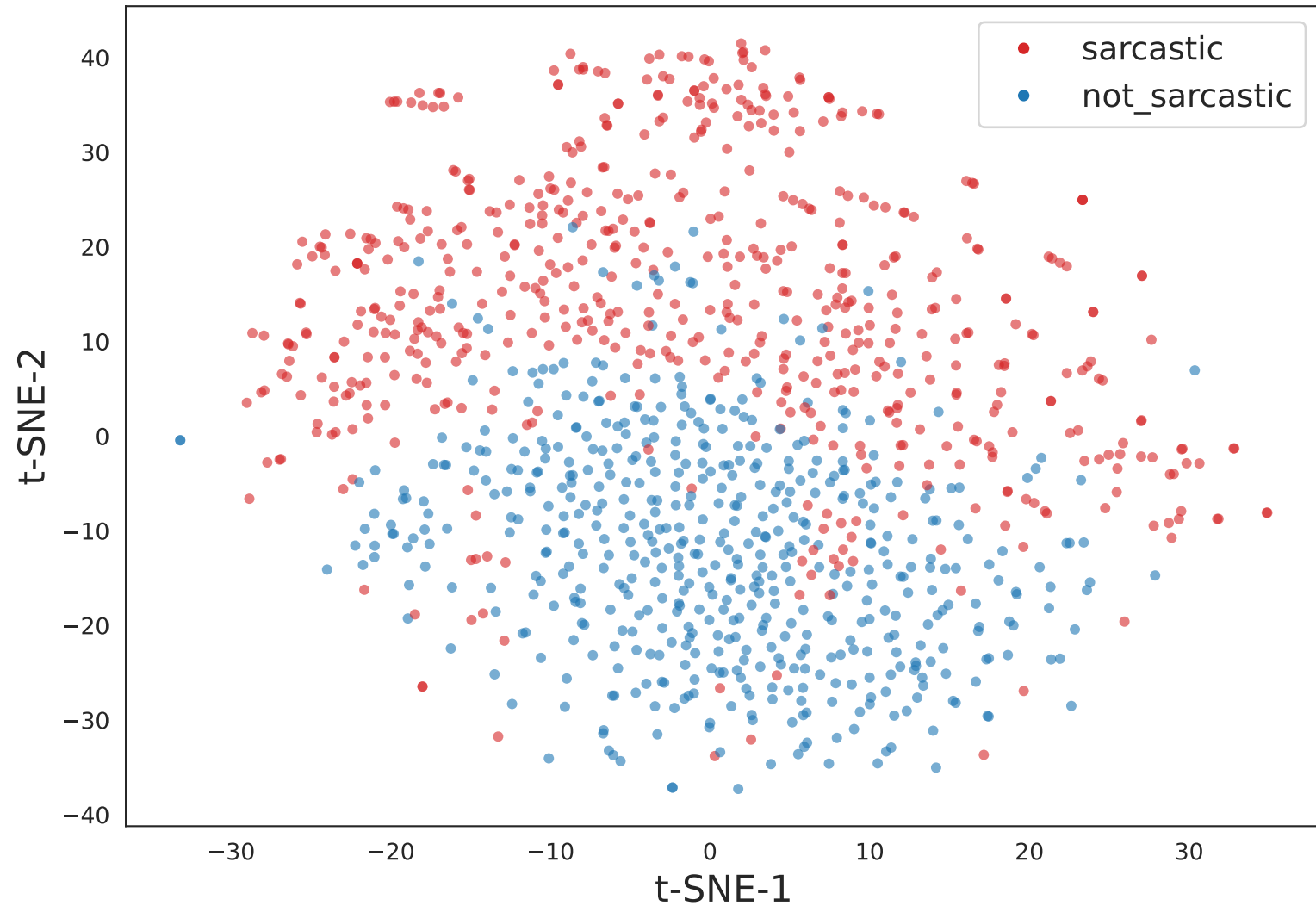
t-SNE 2D
