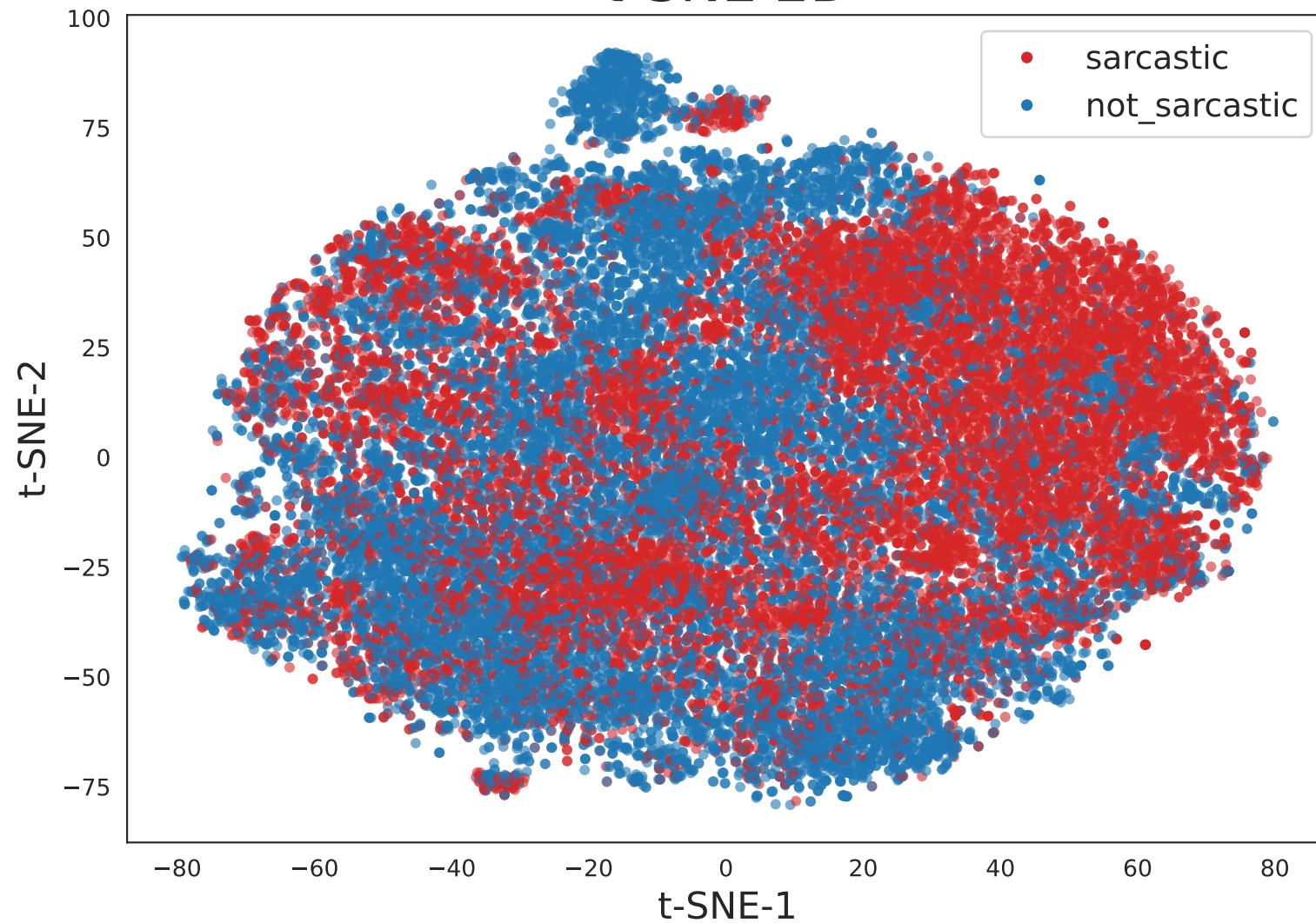
t-SNE 2D
