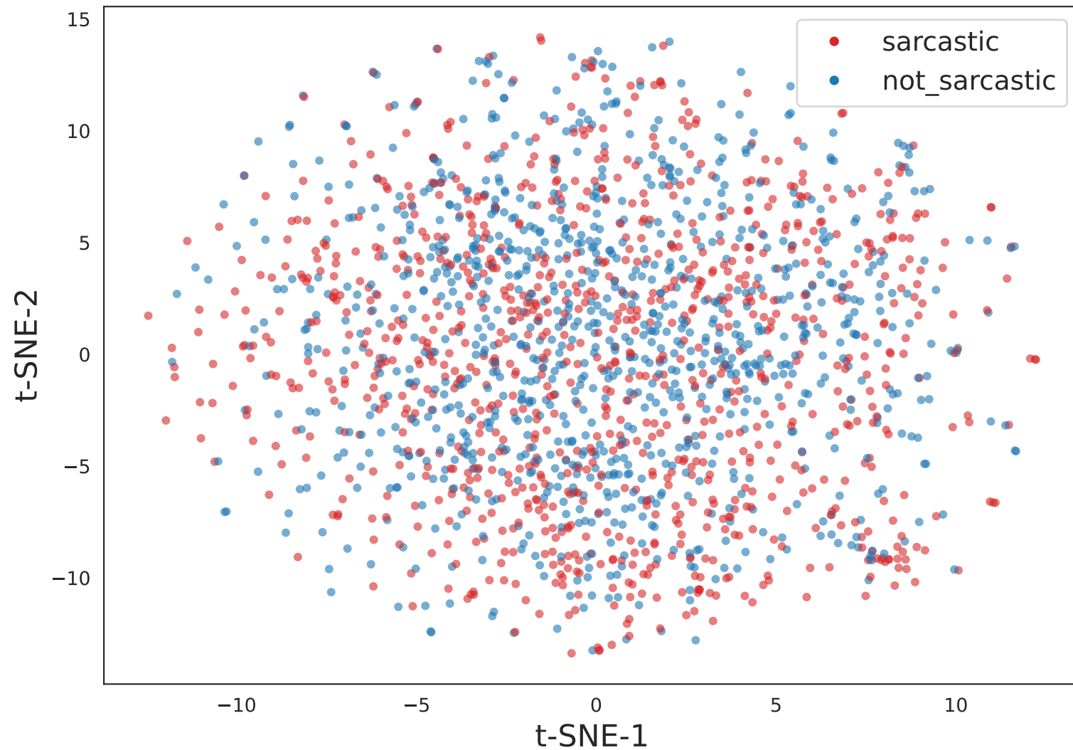
t-SNE 2D
