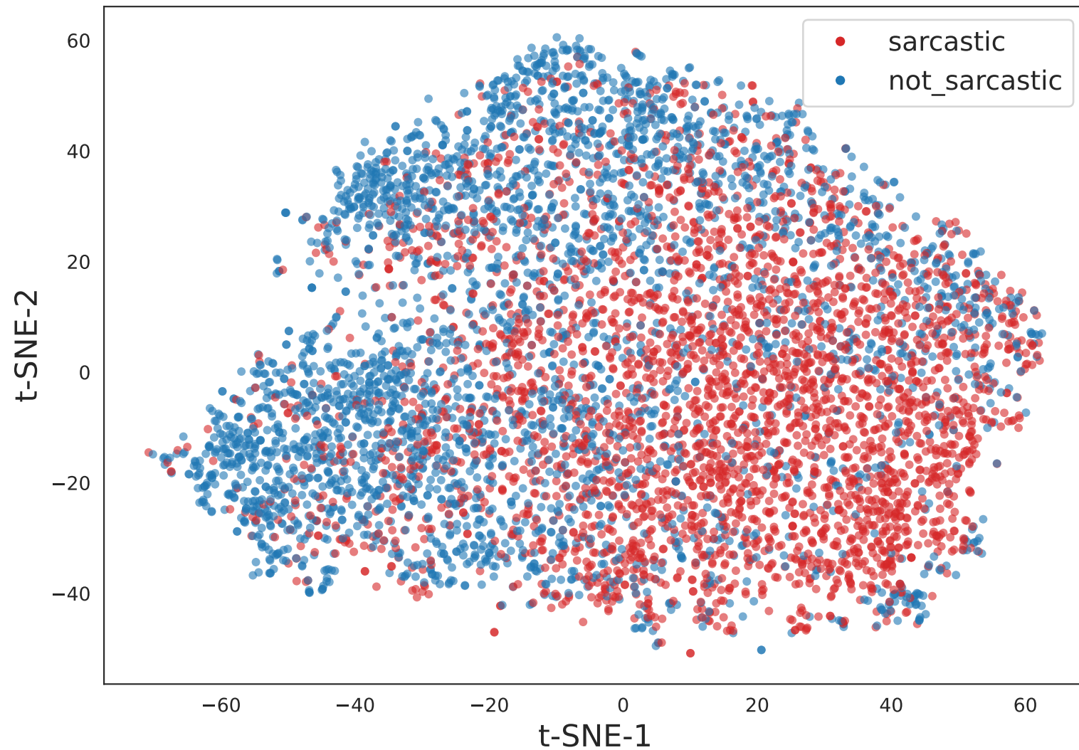
t-SNE 2D
